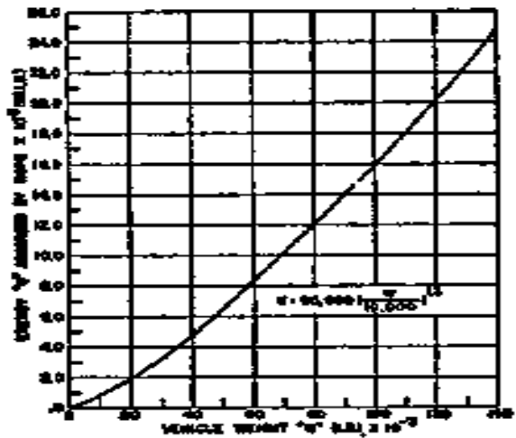
FIGURE W-3—Energy absorbed versus vehicle weight.
